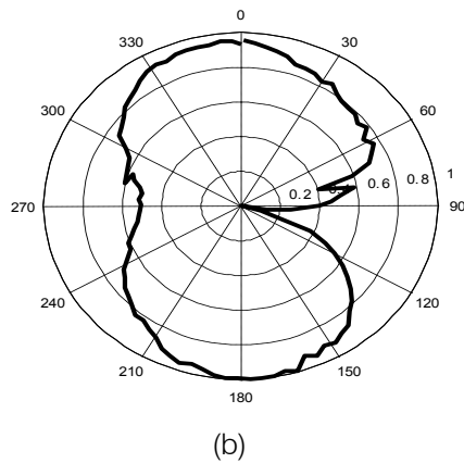
Fig. 6: Measured radiation patterns of (a) conventional MPA and (b) proposed MPA
