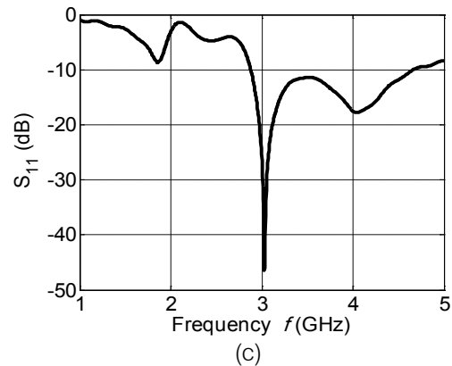
Fig.2: Variation of S_{11} with frequency for (a) Conventional MPA (b) MPA with slotted-patch and the full ground plane (c) Proposed MPA (slotted-patch with modified ground plane).
