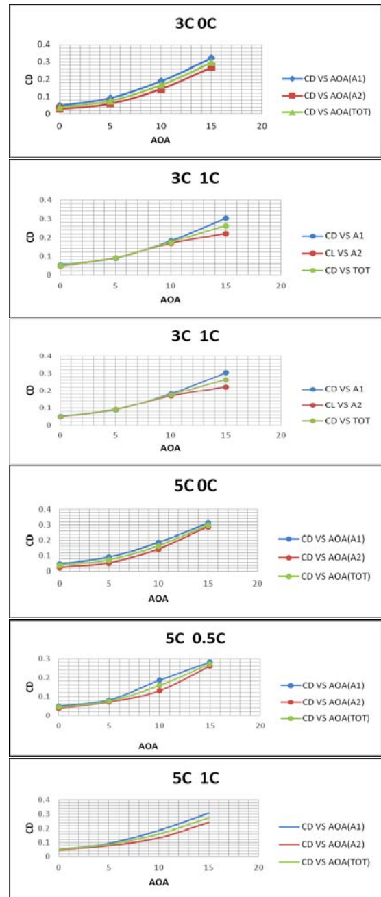
Fig.11: AOA vs C_D for 3c and 5c combinations
