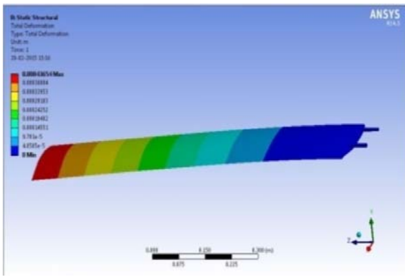
Fig. 15: Structural analysis of wing
