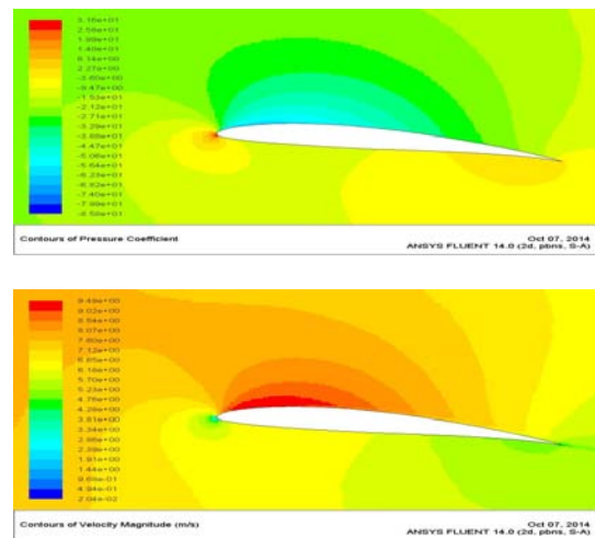
Fig. 9: Contours of pressure coefficient and Velocity magnitude
