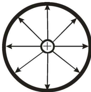
Fig. 1 : The liquid-drop model of atom.
