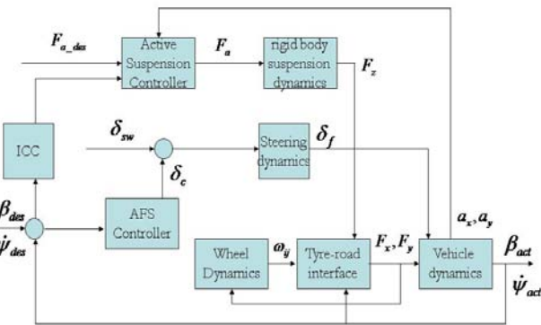
Fig. 21 : Schematic of ICC strategy between AFS & AS
