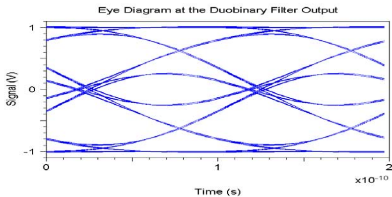
Figure 12 : Eye Diagram
