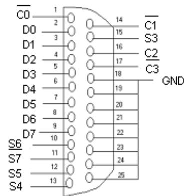
Figure 15 : Pin Configuration of the parallel port
