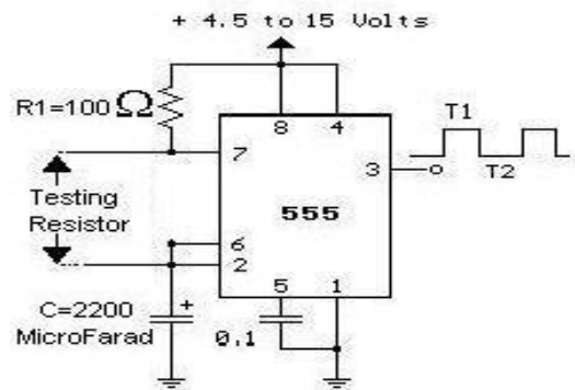
Figure 9 : Measuring the Resister
