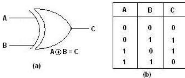
Figure 2 (a) : Symbol and (b)truth table for EXOR gate
