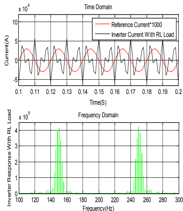
Figure 7 : Inverter Response with RL Load
