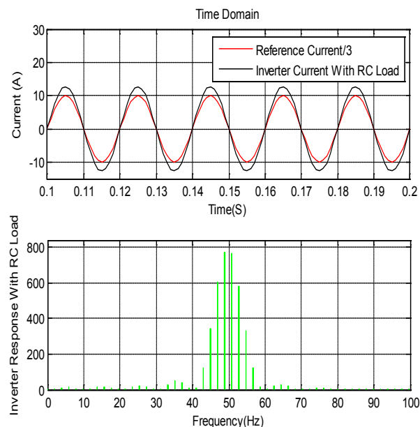
Figure 11 : Inverter Response with RC Load
