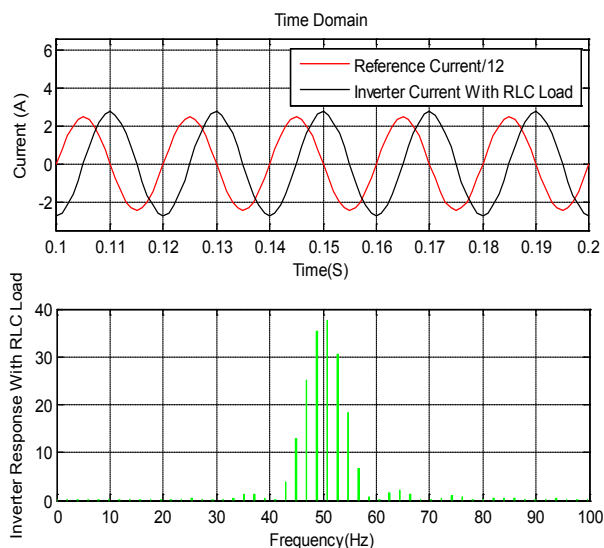
Figure 9 : Inverter Response with RLC Load
