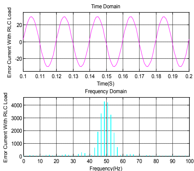
Figure 10 : Error Current with RLC Load
