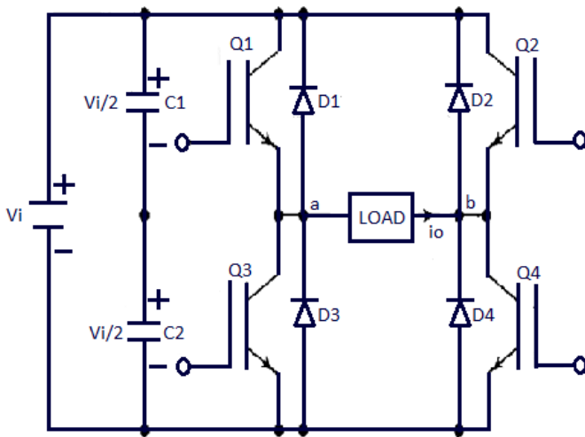
Figure 2 : Circuit Diagram of a Full Bridge Inverter
