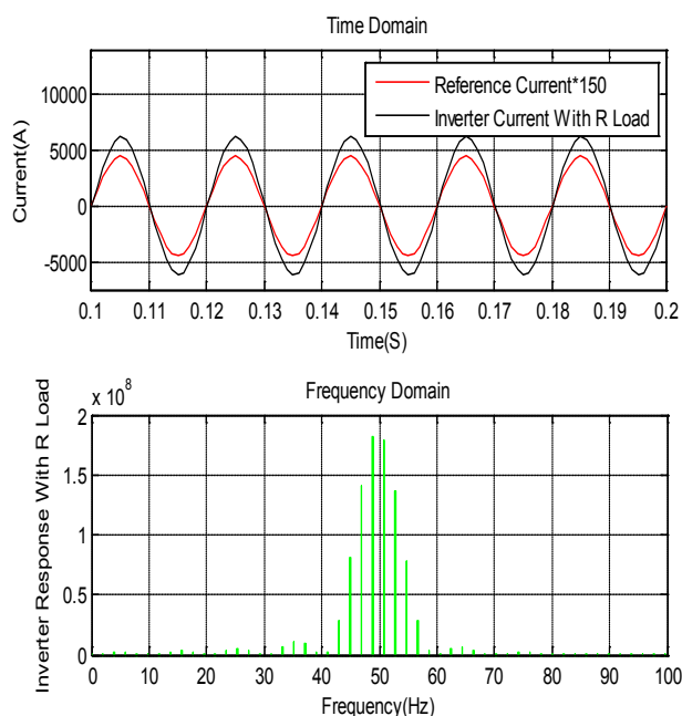
Figure 5 : Inverter Response with R Load
