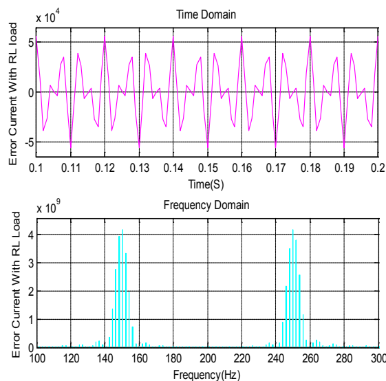
Figure 8 : Error Current With RL Load
