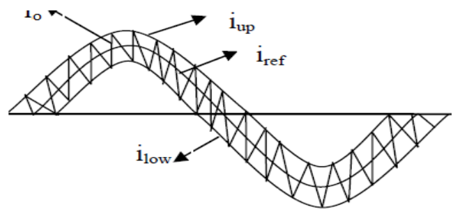
Figure 4 : Delta Modulation Structure [10]
