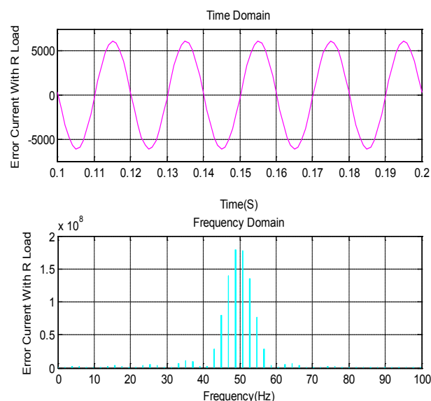
Figure 6 : Error Current With R Load
