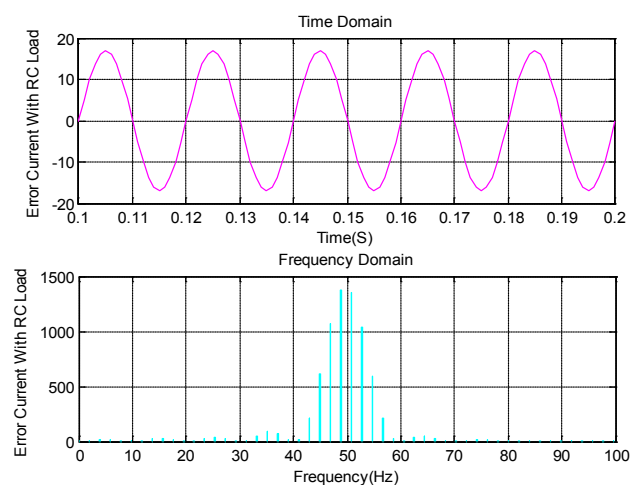
Figure 12 : Error Current with RC Load
